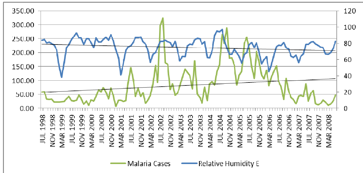
Figure 24 Relationship between malaria and relative humidity of evening
