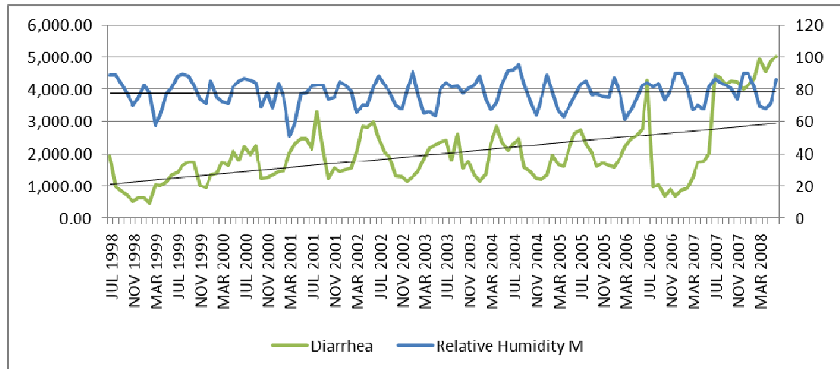
Figure 28 Relationship between diarrhea and morning relative humidity
