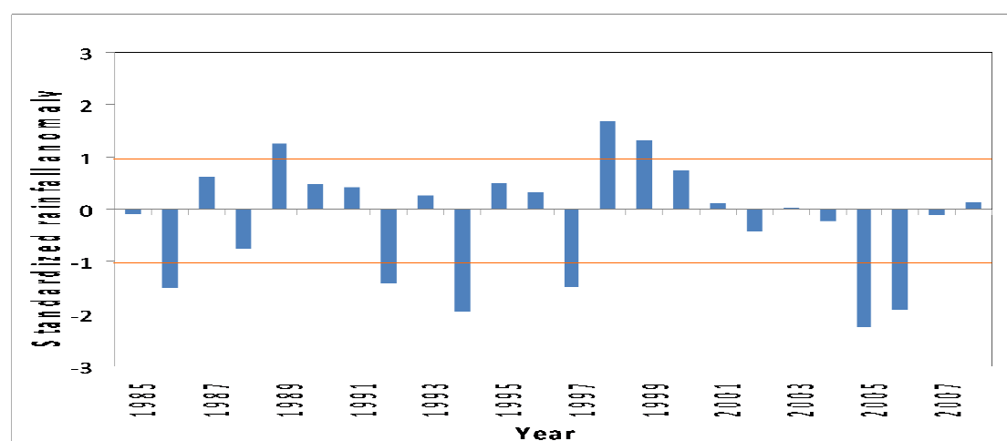
Figure 19 Inter-annual variation of annual total rainfall
