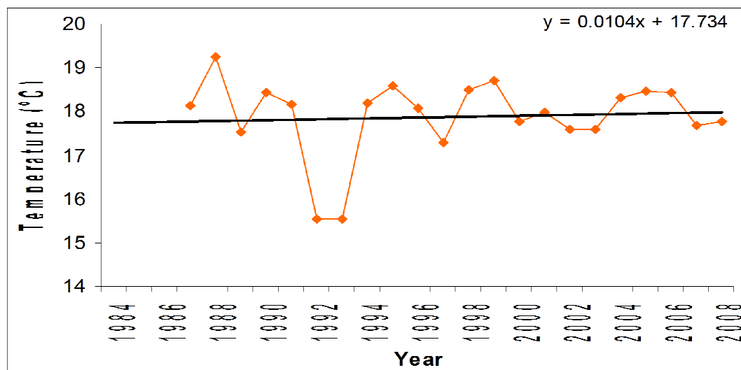
Figure 15 Annual minimum temperature trend
