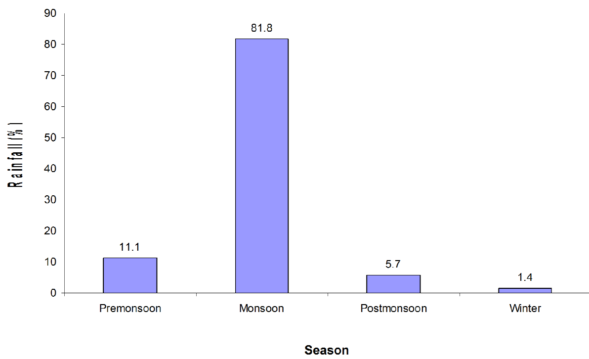
Figure 11 Seasonal contributions in total annual rainfall
