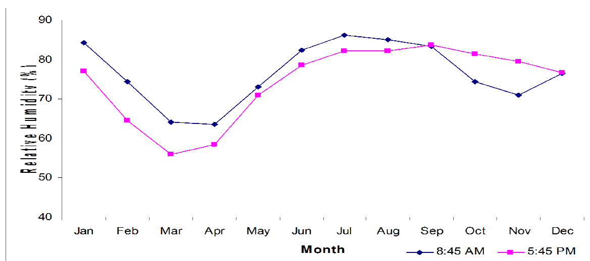
Figure 12 Monthly variation of relative humidity in Jhapa
