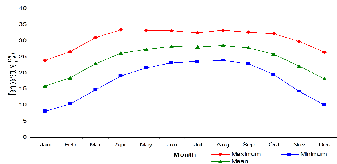
Figure 7 Monthly variation of temperature in Jhapa
