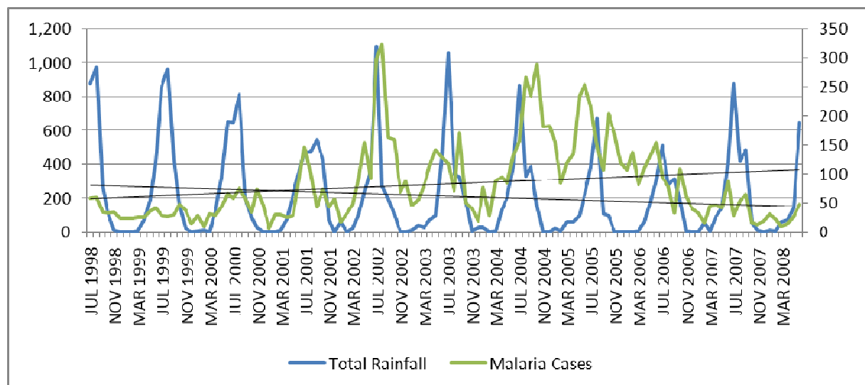
Figure 25 Relationship between malaria and total rainfall
