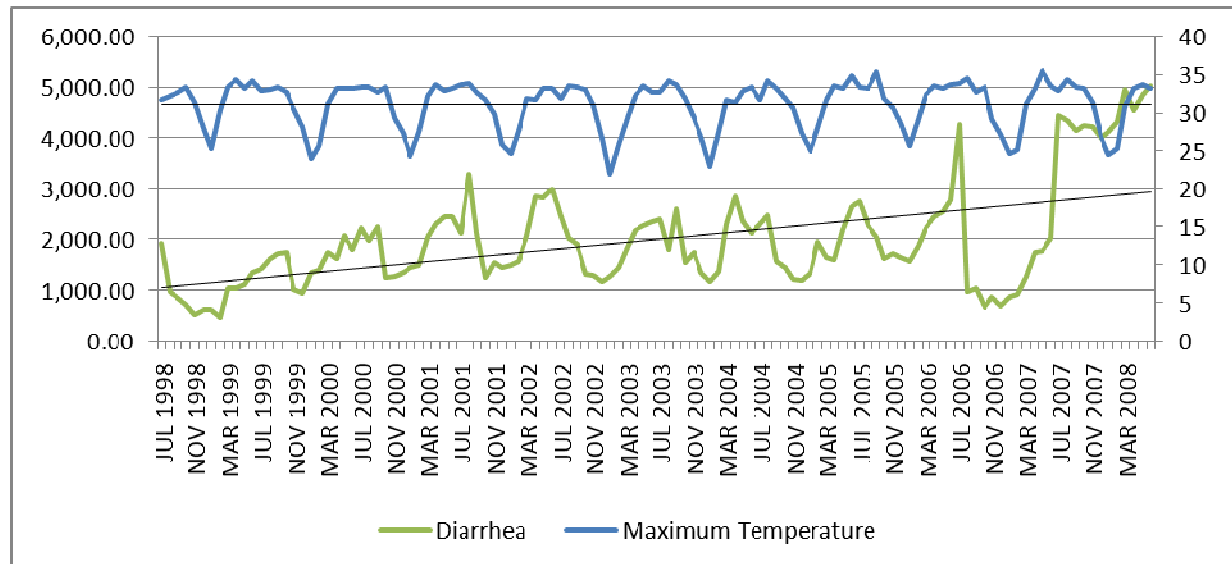
Figure 26 Relationship between diarrhea and maximum temperature
