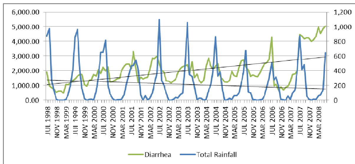
Figure 30 Relationship between diarrhea and total rainfall
