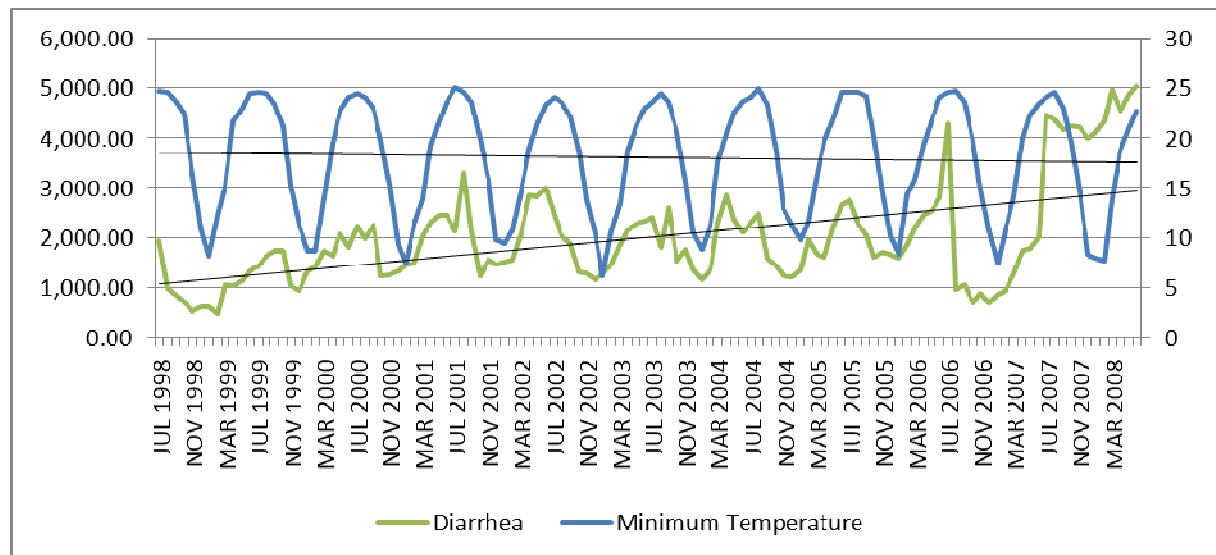
Figure 27 Relationship between diarrhea and minimum temperature
