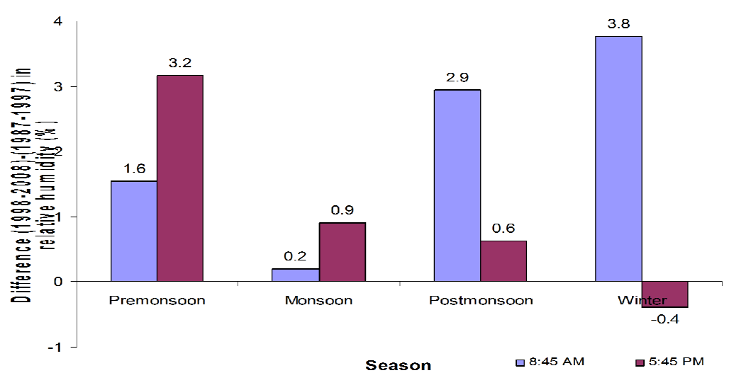
Figure 20 Decadal change in RH (1998-2008) - (1987-1997)
