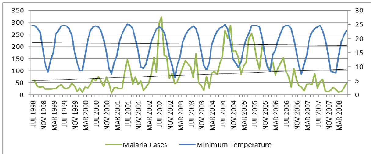
Figure 22 Relationship between Malaria and Minimum Temperature
